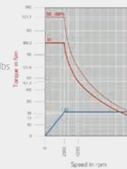
Power / Torque Diagram
