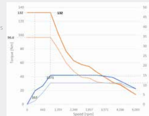
Spindle Power / Torque Diagram
